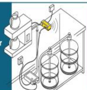
Coffee Cart / Kiosk with Dual Inlet BW System and Appliance Controller
